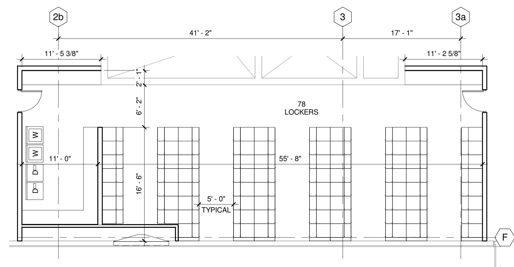
NORTH 2 ENLARGED FLOOR PLAN 1/8" = 1'-0"
