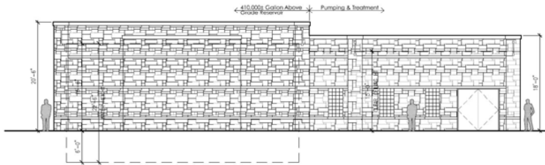
1 PROPOSED FRONT ELEVATION
