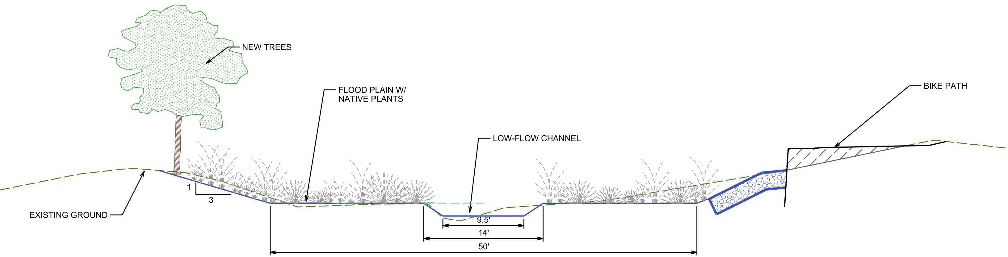
TYPICAL SECTION: CHANNEL
